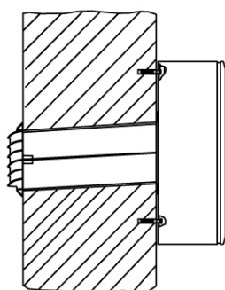
On-wall installation
