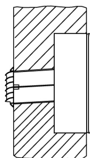
In-wall installation
